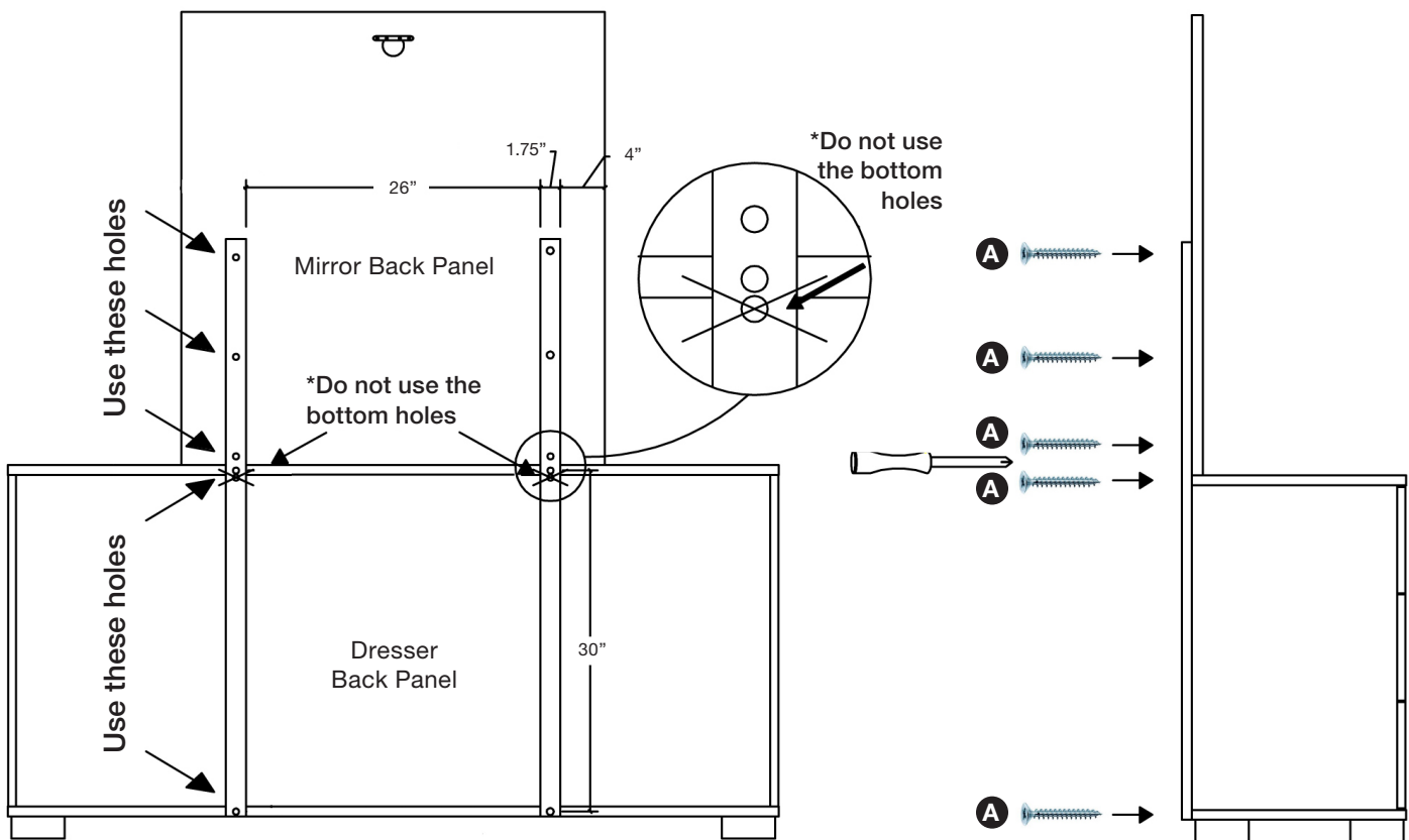
REAR VIEW
