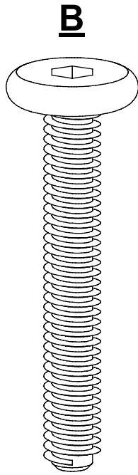
M6*45 4 PCS
