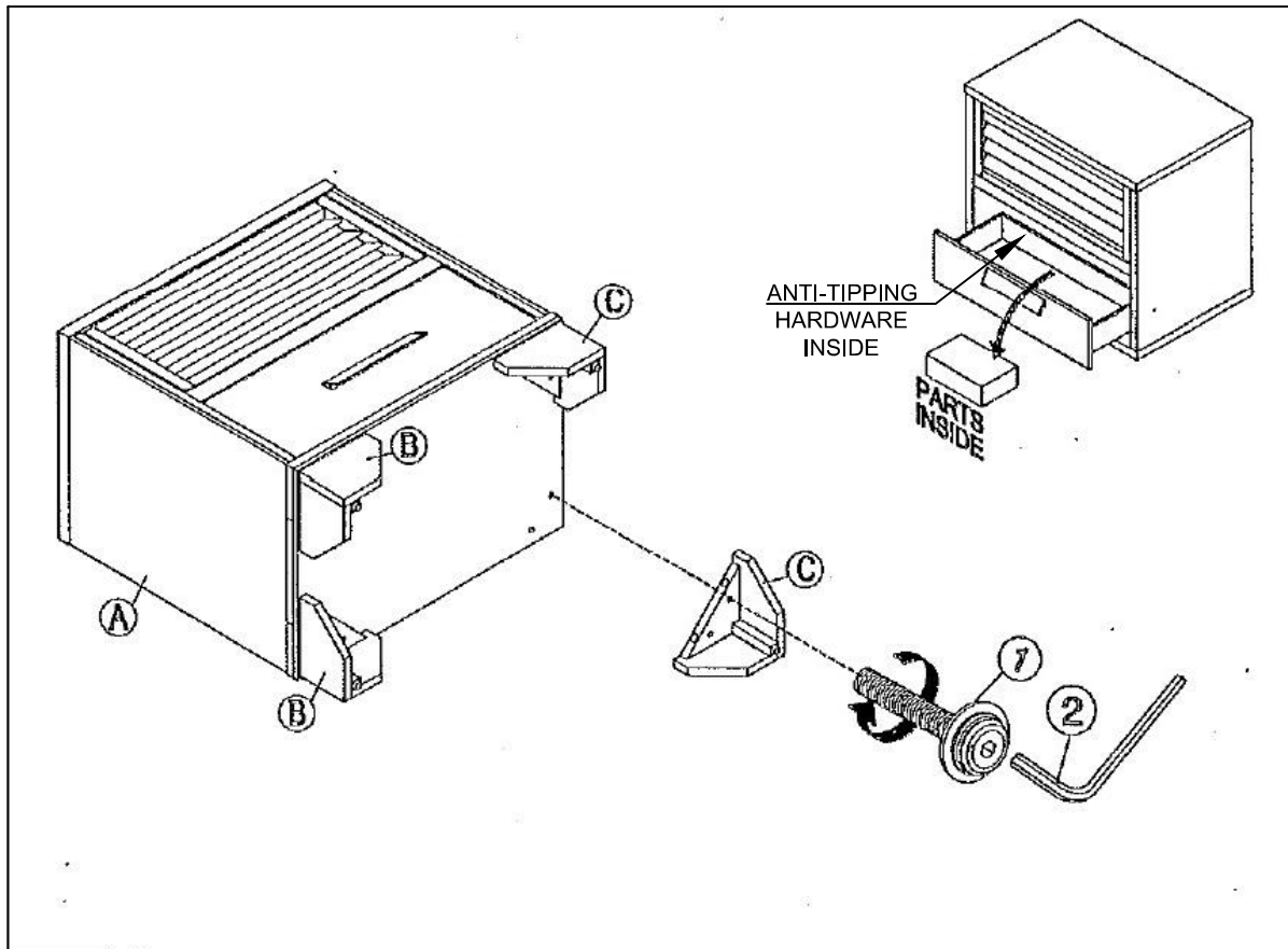
COMPLETED NIGHTSTAND ASSEMBLY
