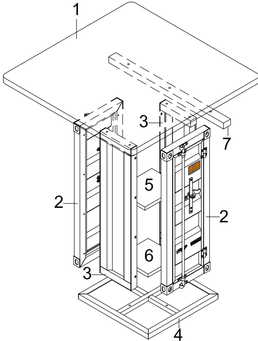
Exploded View
