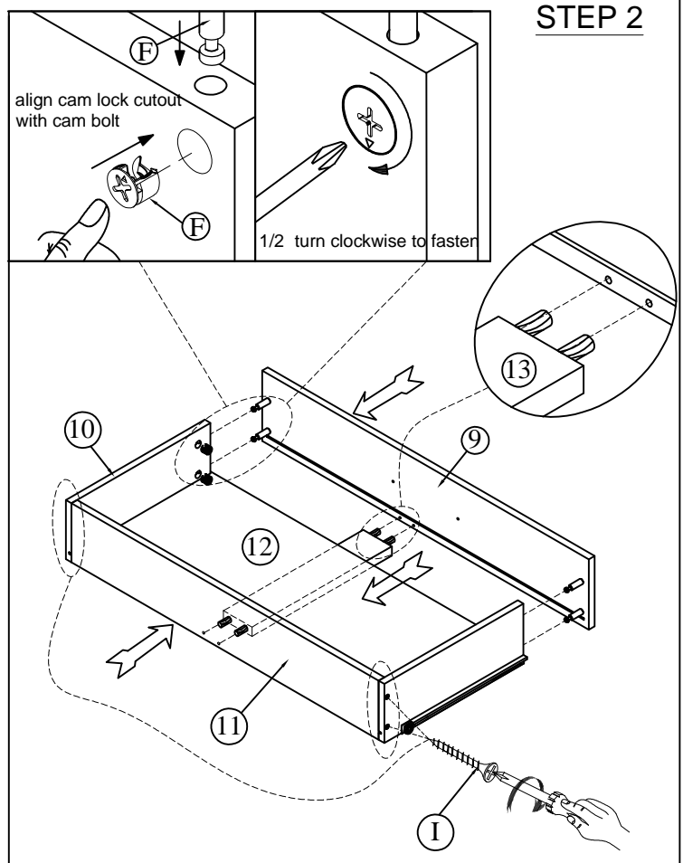
Completed Drawer
